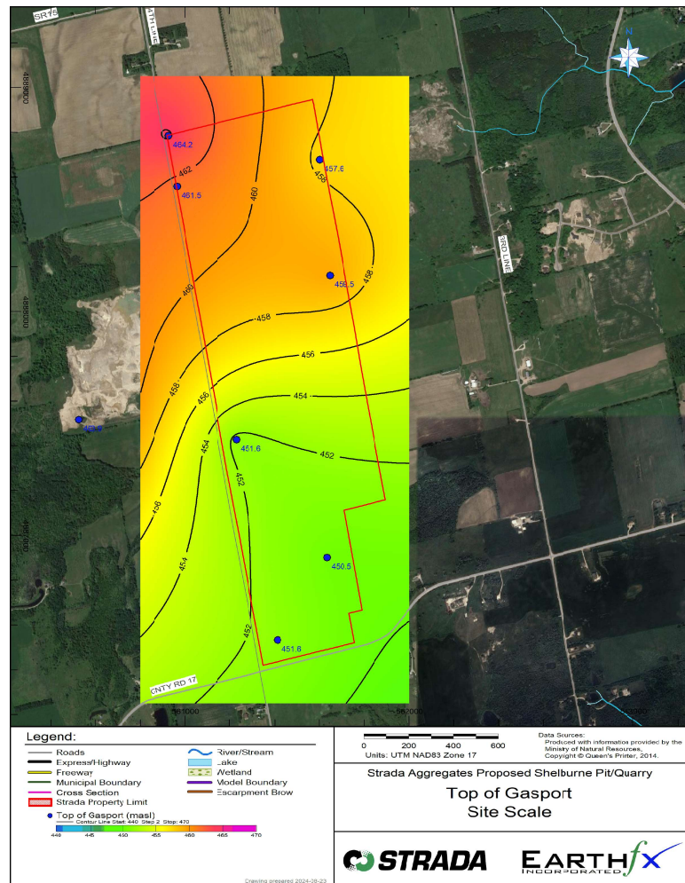
Figure 3.33: Top of Gasport - Site Scale
