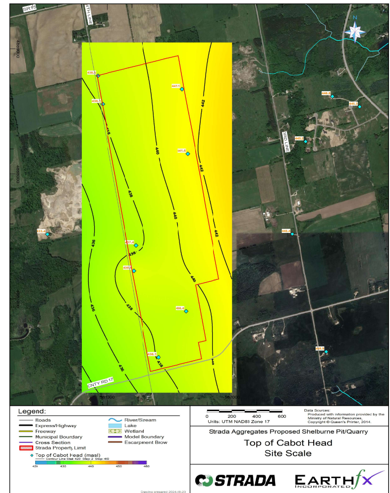
Figure 3.34: Top of Cabot Head - Site Scale
